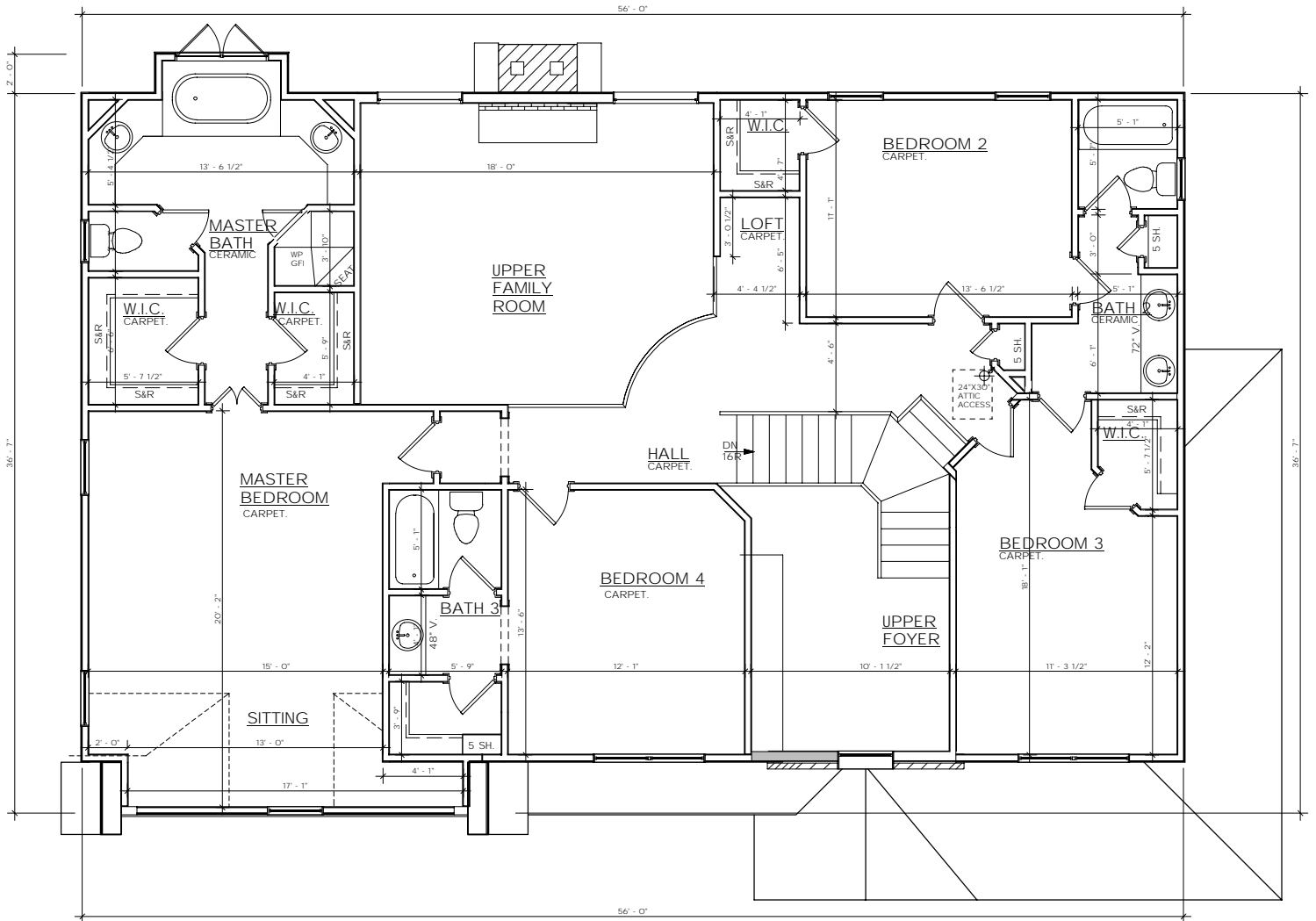
SECOND FLOOR PLAN 9'-0" CEILING
