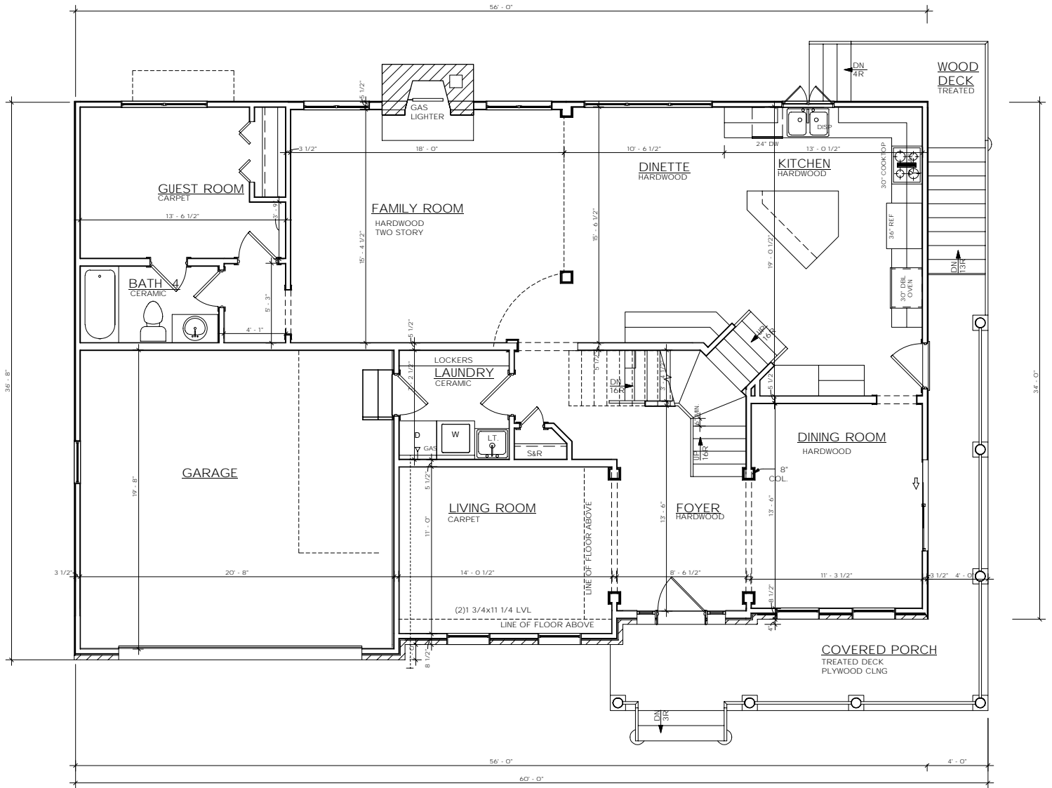
FIRST FLOOR PLAN 9'-0" CEILING
